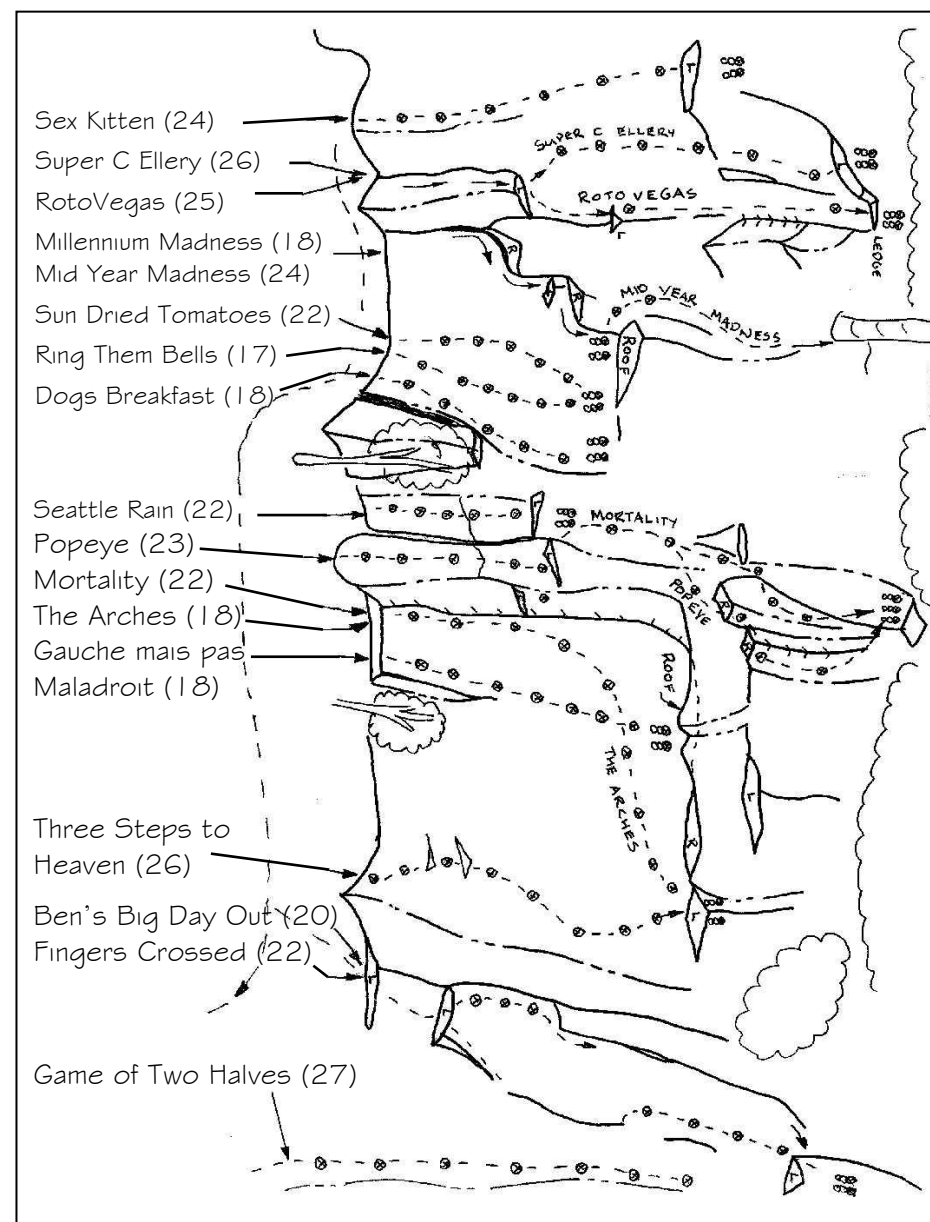
Figure 2: Main Cliff
